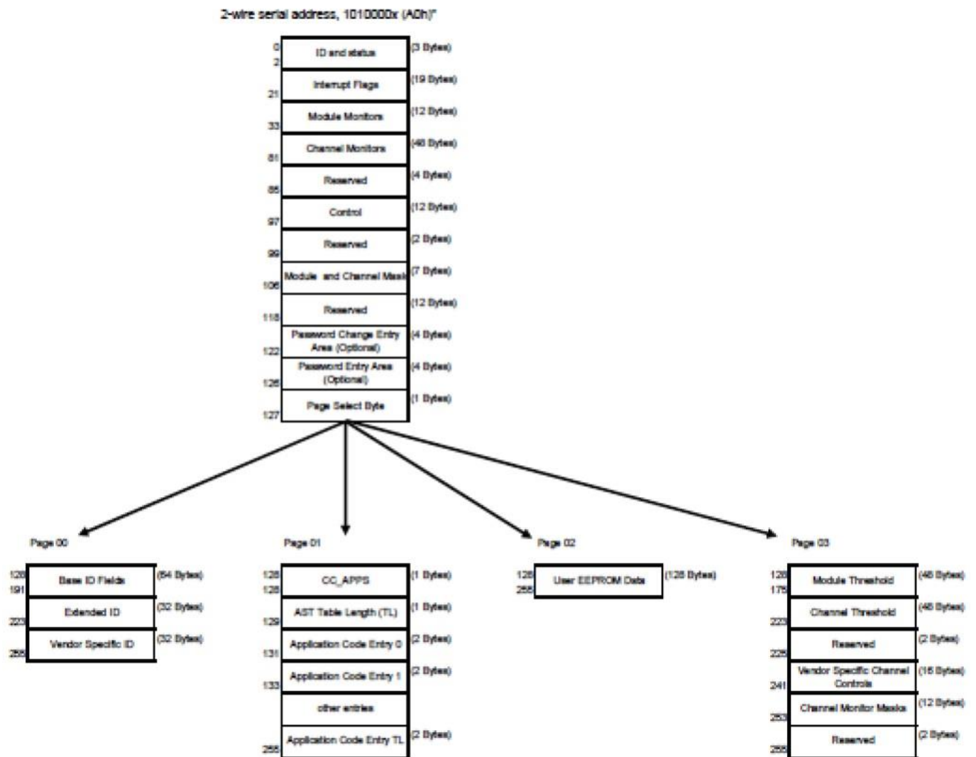
Figure 2 –QSF+ Memory Map
