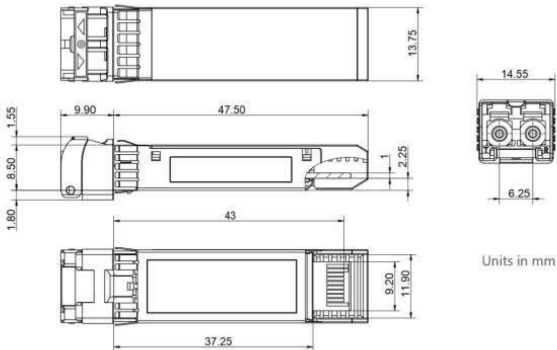
Mechanical Outline
